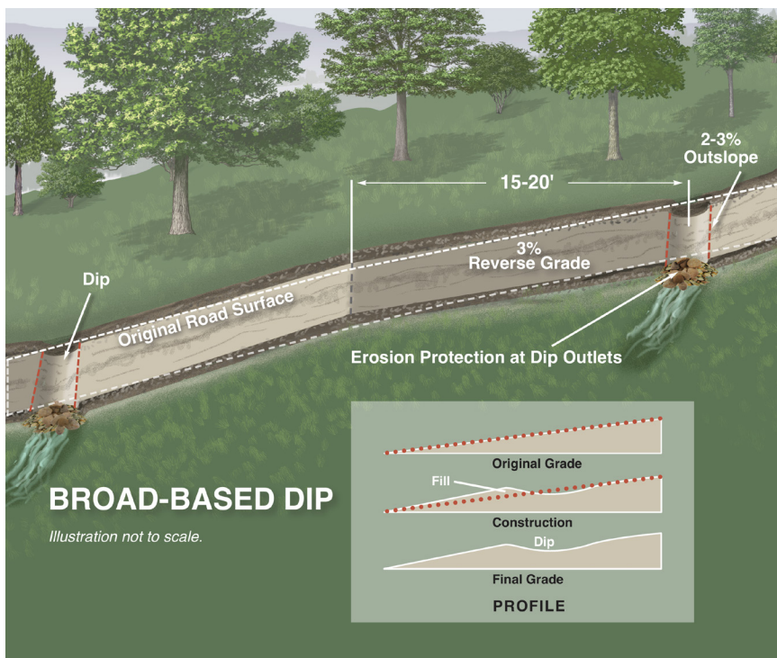
Figure 4. Broad-based dip
