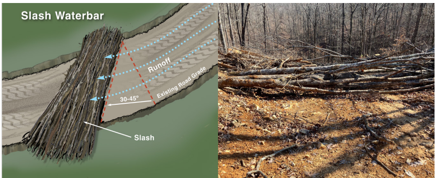
Figure 7b. Water bar construction
