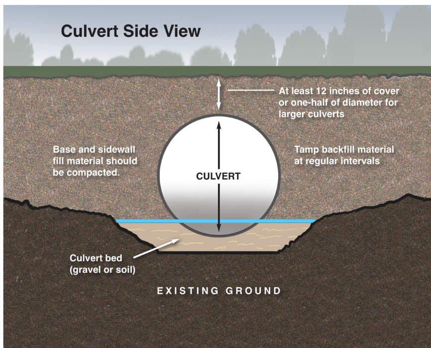
Figure 6. Culvert side
